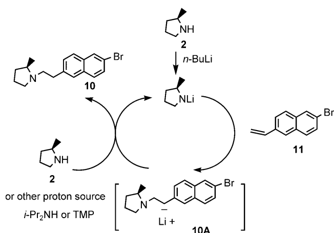
Scheme 3. Proposed hydroamination pathway.
