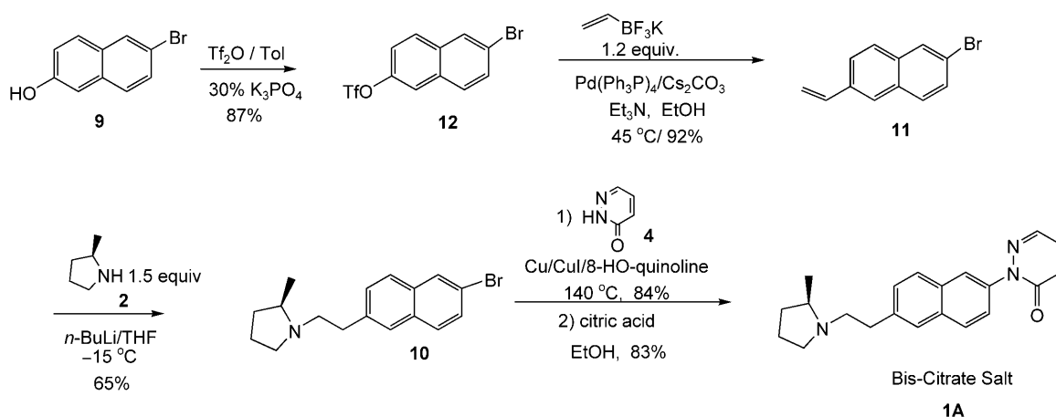
Scheme 4. The new four-step process.
