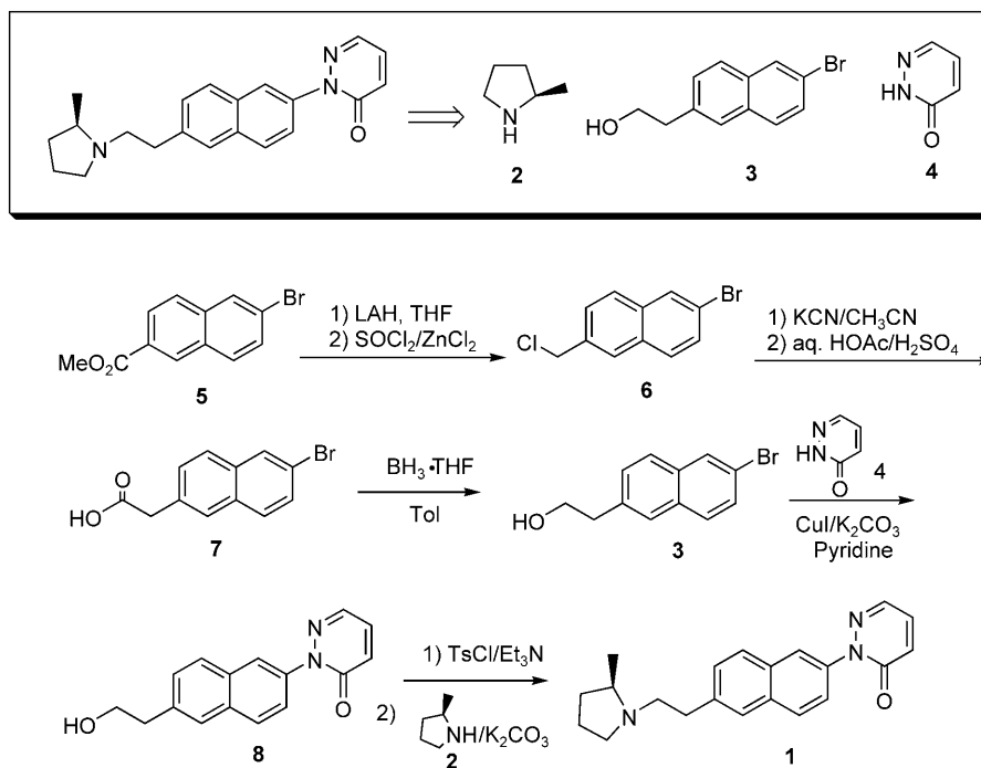
Scheme 1. The initial eight-step process.
